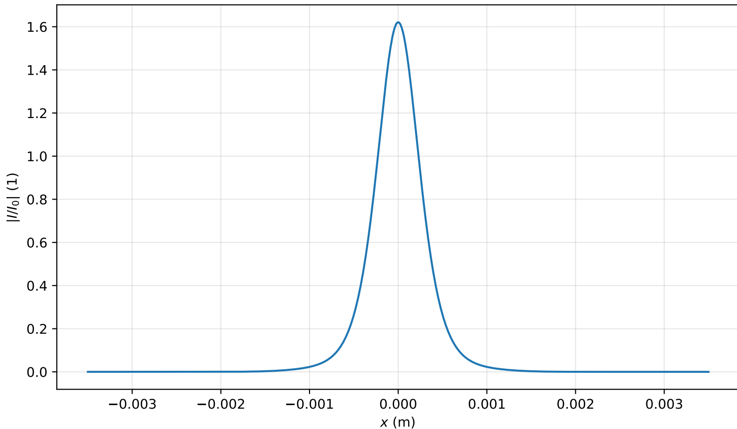
Intensity profile I(x, y = 0, z = 1.831m)/I_0 , P_{in}=0.9P_{cr} , artificial time
